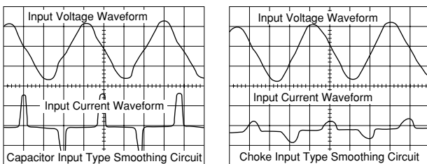
Fig. 2 Input vltage-current curves
