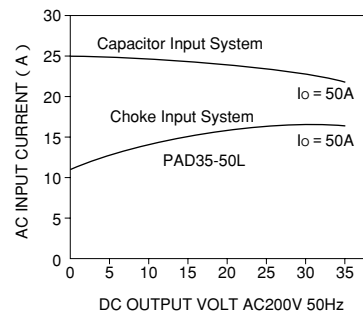
Fig.3 Current Consumption Characteristics
