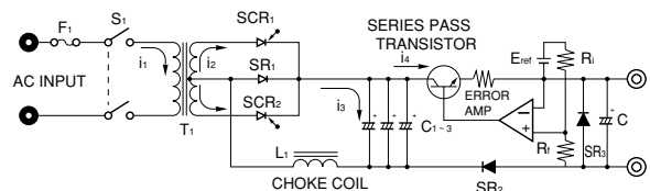
Fig. 5 Basic Circuitry of the PAD-L Series
